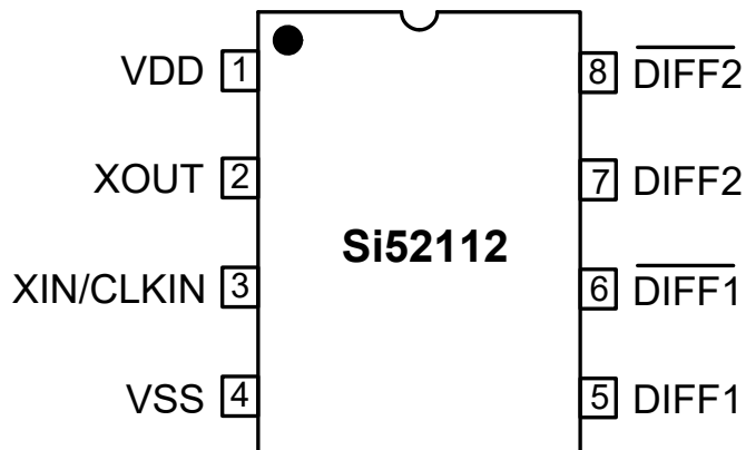
Figure 7. 8-Pin TSSOP
