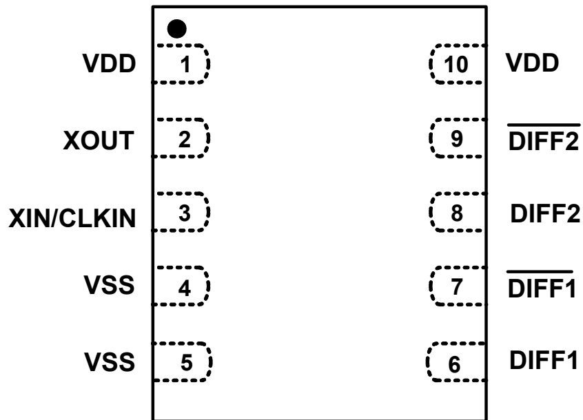
Figure 6. 10-Pin TDFN
