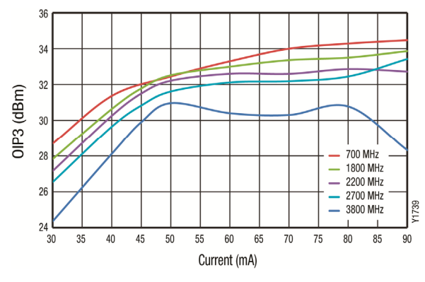
Figure 16. OIP3 vs Quiescent Current over Frequency
