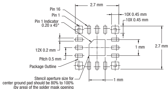
Stencil Aperture
