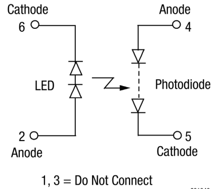
Figure 1. OLS910 Block Diagram
