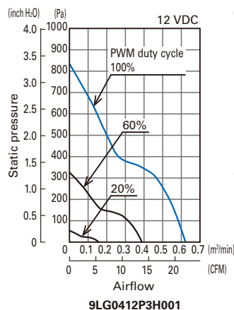
PWM duty cycle
