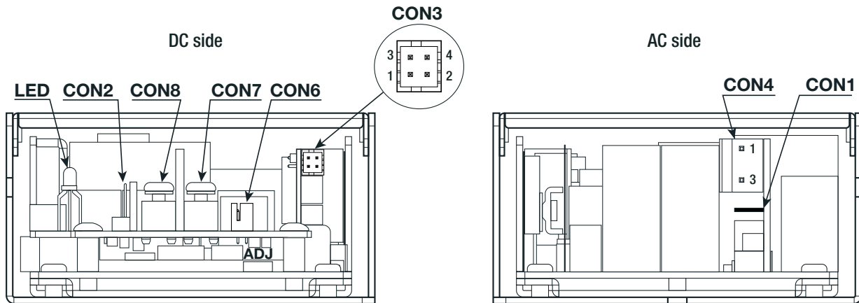
Dimension Drawing Enclosed Version (mm)
