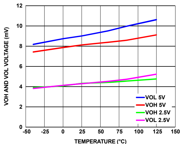
FIGURE 28. PGIA V_OH AND V_OV vs TEMPERATURE
