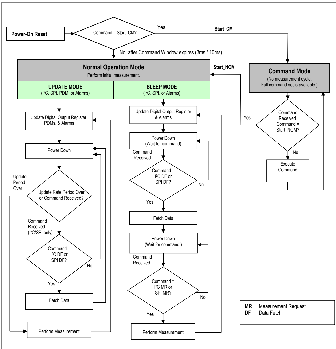
Figure 10. General Operation
