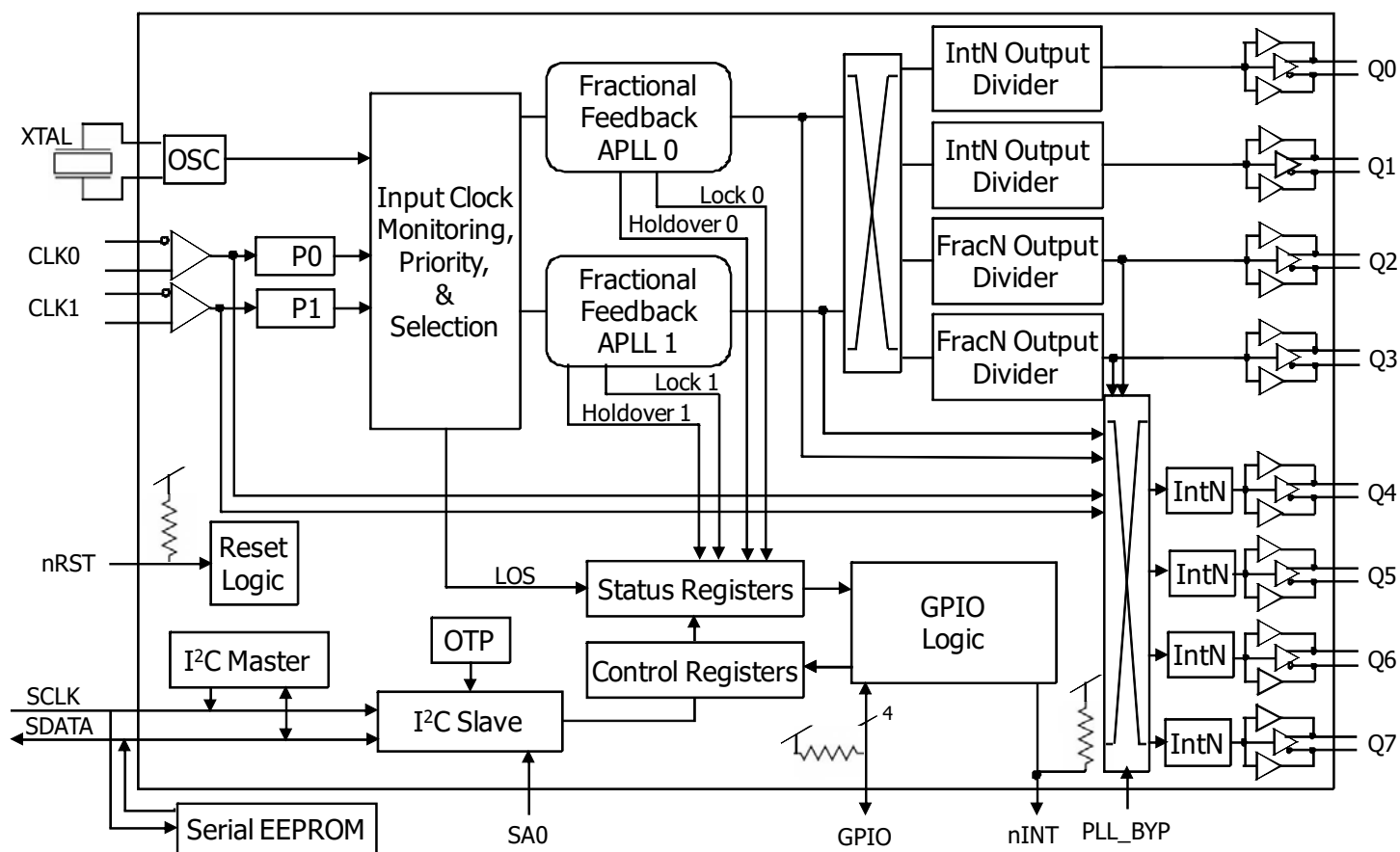
Figure 1. 8T49N287 Functional Block Diagram
