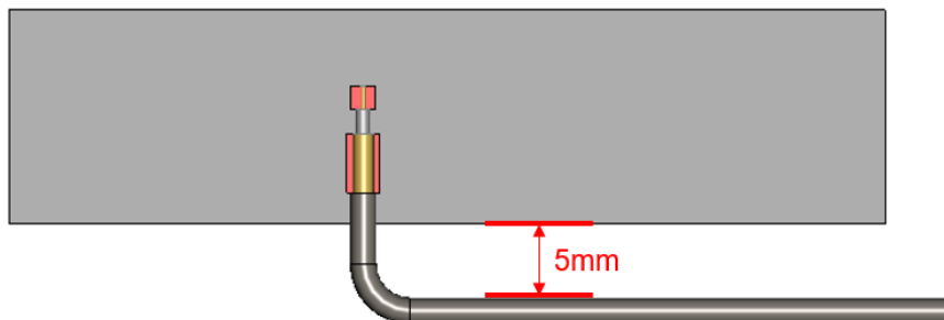
Figure 1 Cable Bending
