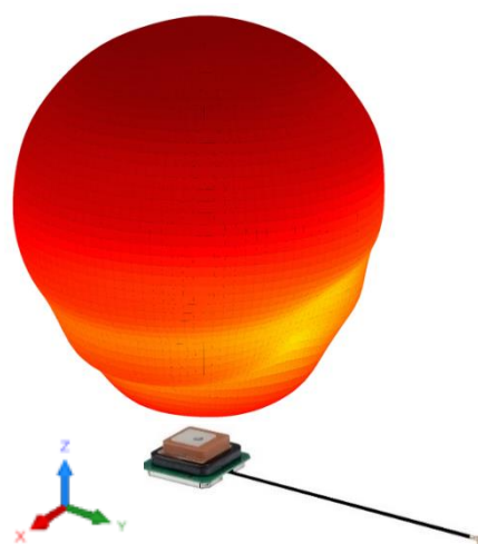
L5 3D RHCP Pattern @1176 MHz
