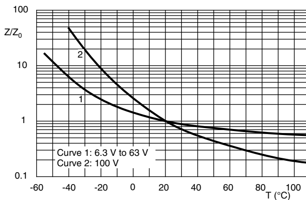
Fig. 11 - Typical multiplier of impedance Z as a function of temperature at 100 kHz
