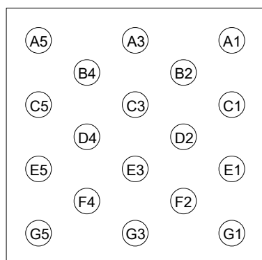
Ball-side View
