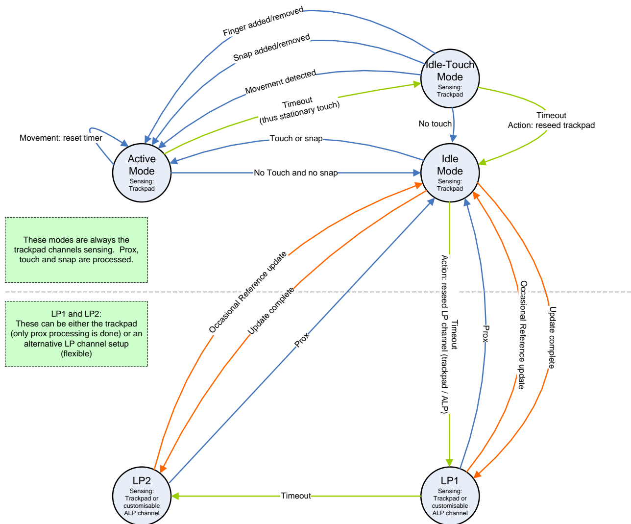
Figure 4.1 System Mode State Diagram
