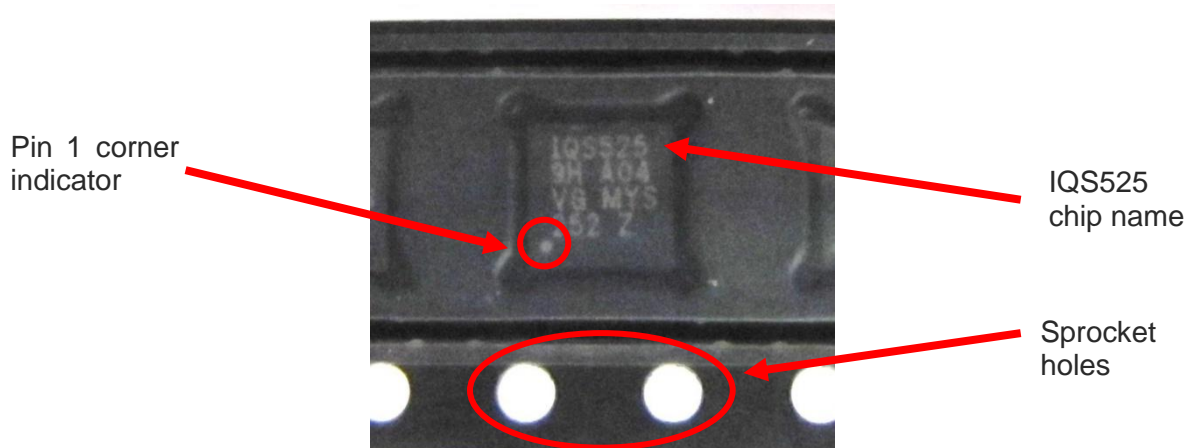
Figure 12.3 IQS525 QFN28-4x4 Package in Carrier Tape Example
