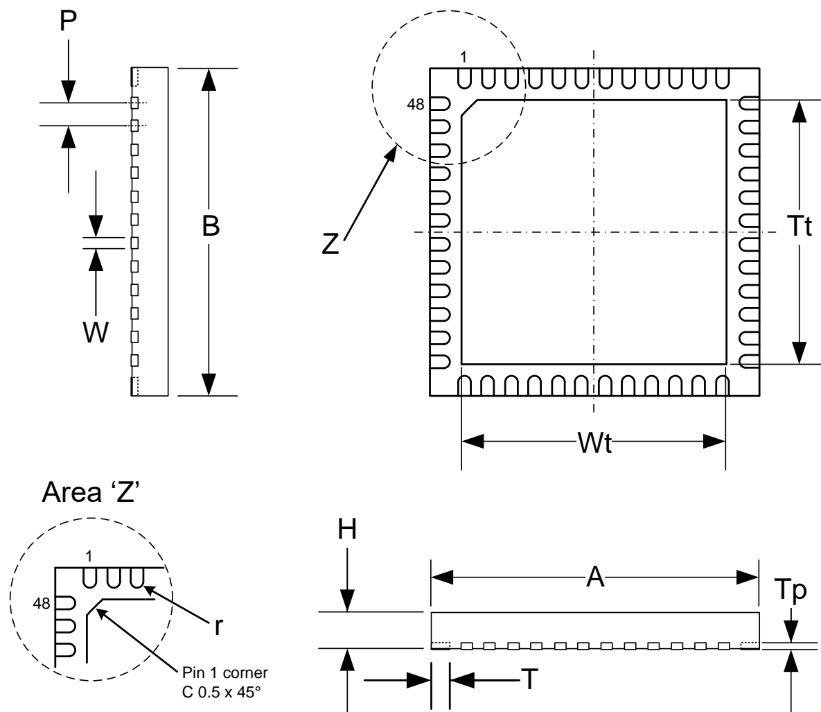
Figure 11.1 QFN(7x7)-48 Package
