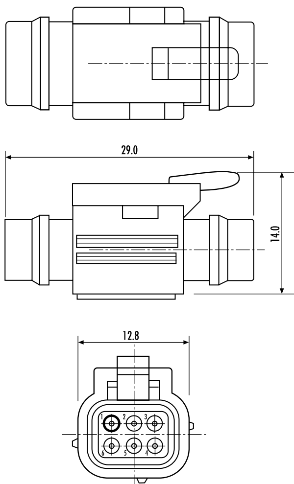
MATED PAIR
