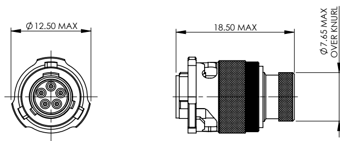
PLUG - TYPE 6
