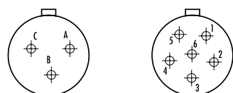
INSERT ARRANGEMENTS
