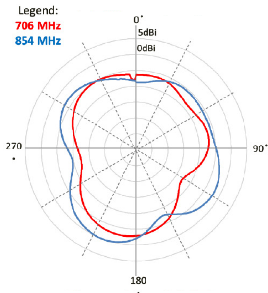
Azimuth(XY)
