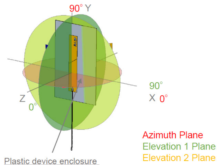
Test setup
