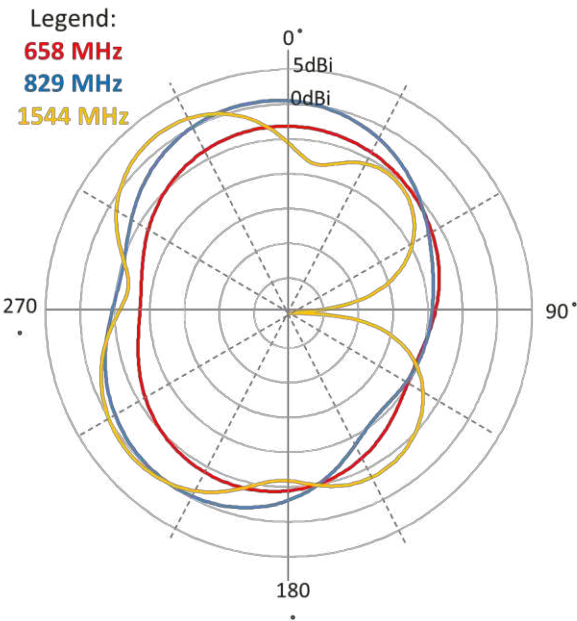
Elevation 1(XZ)
