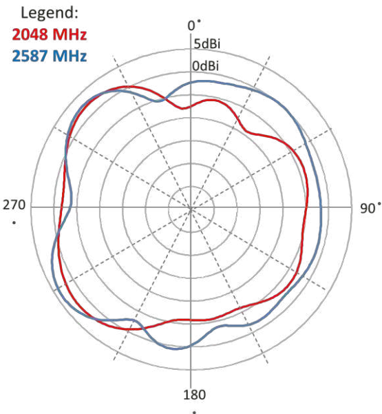
Elevation 1(XZ)
