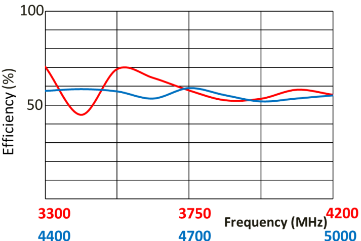
Efficiency
