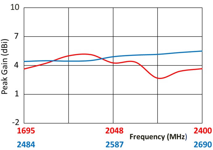
Peak Gain
