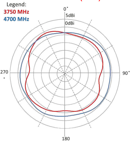
Elevation 2(YZ)
