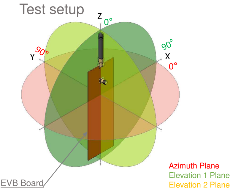
Elevation 1(XZ)
