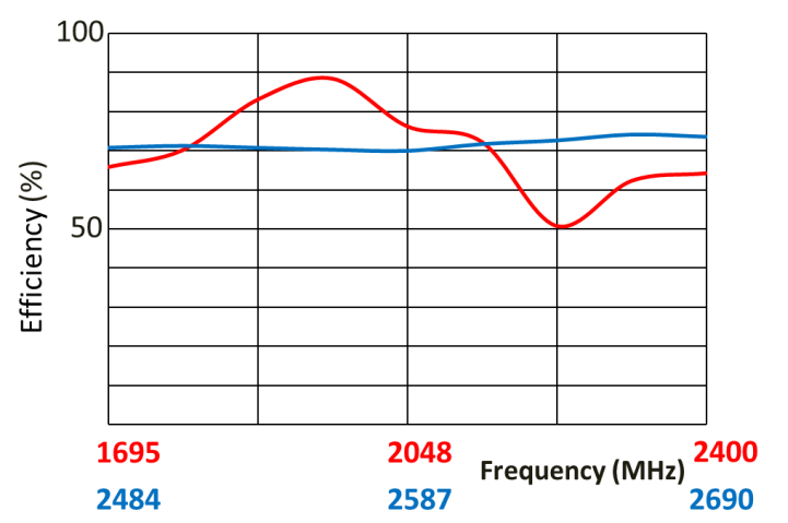
Efficiency
