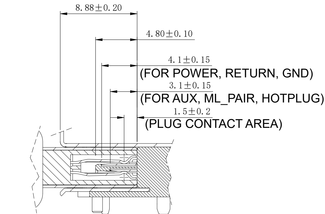
CONNECTOR MATING DIAGRAM
