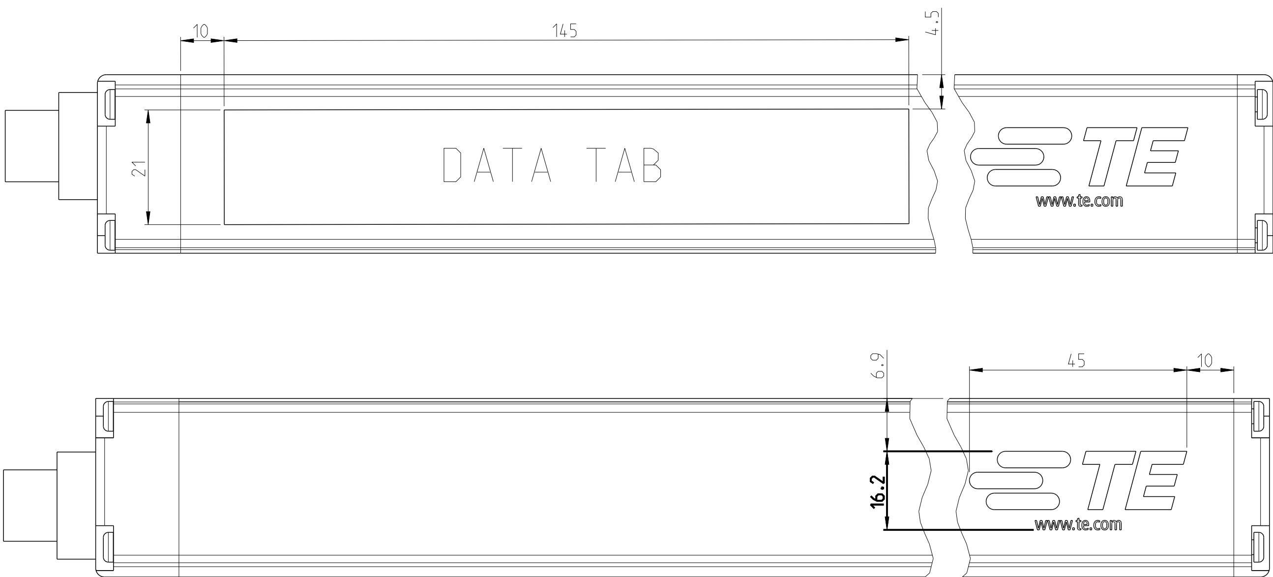
LIGHT CURTAINS RECEIVER-Models with length >15x
