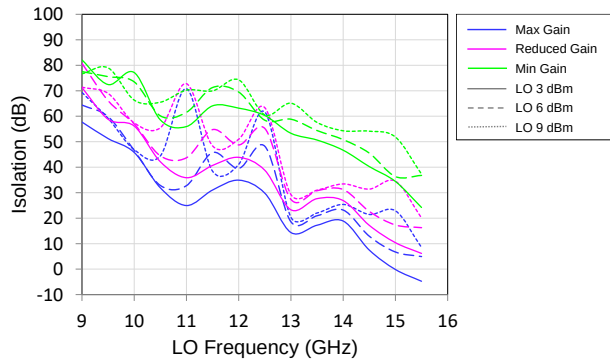
LSB LO-to-RF Isolation vs. LO Freq vs. LO Power and State
