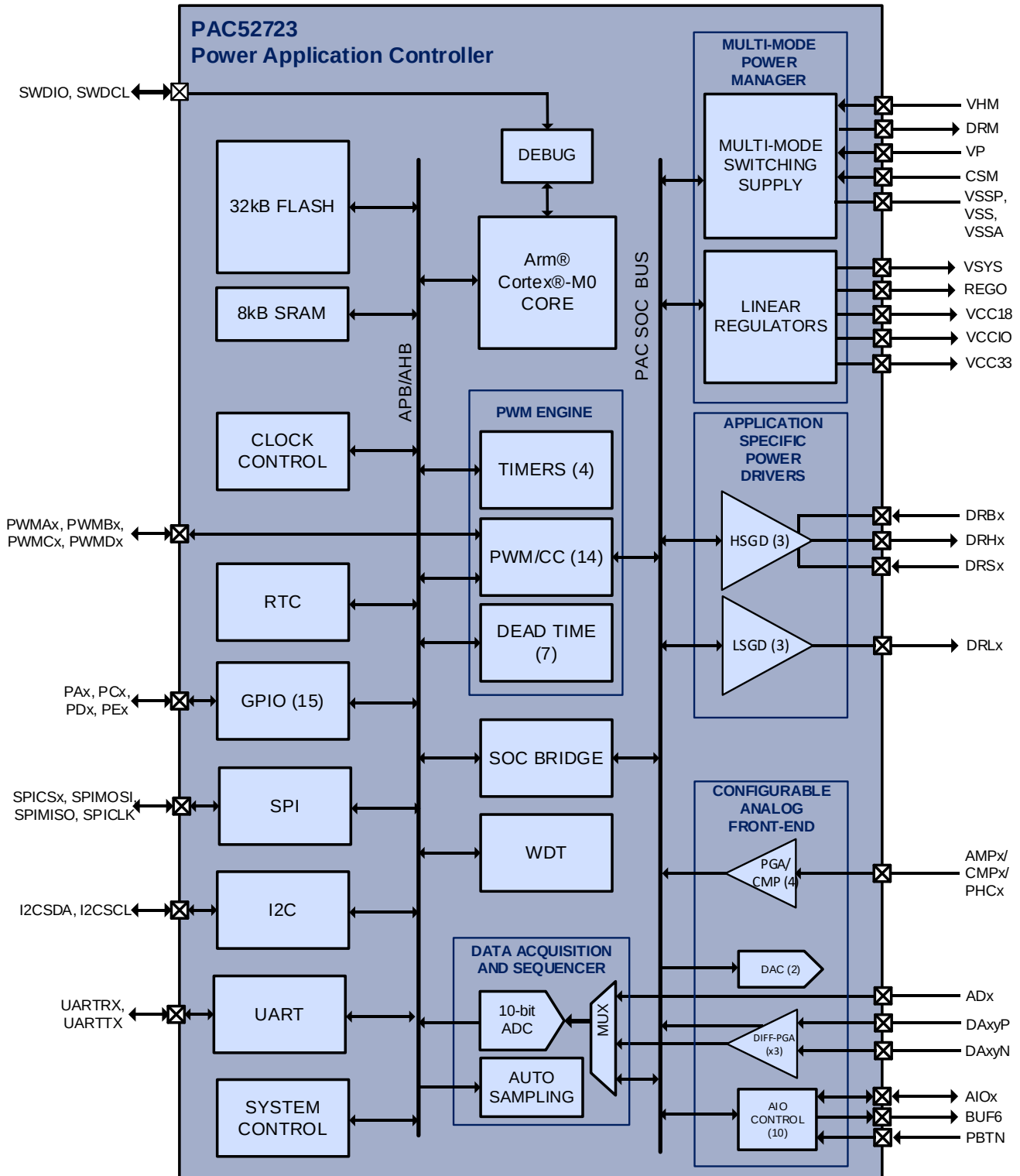
Figure 7-1 PAC52723 Architectural Block Diagram
