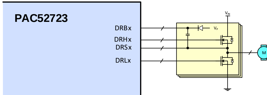
Figure 12-2 Typical Gate Driver Connections
