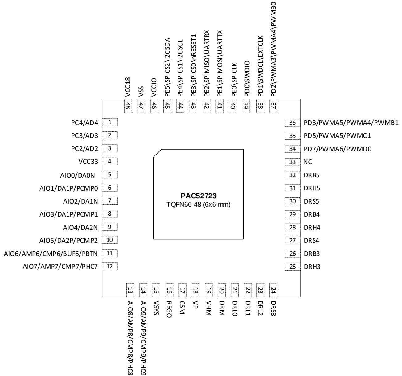
Figure 8-1 PAC52723 Pin Configuration (TQFN66-48 Package)
