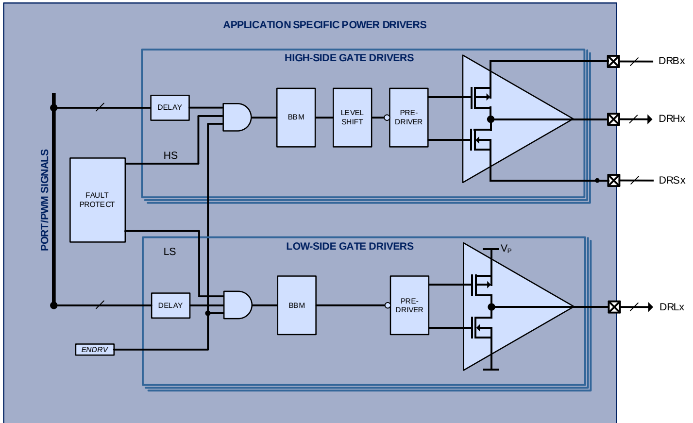
Figure 12-1 PAC52723 Application Specific Power Drivers
