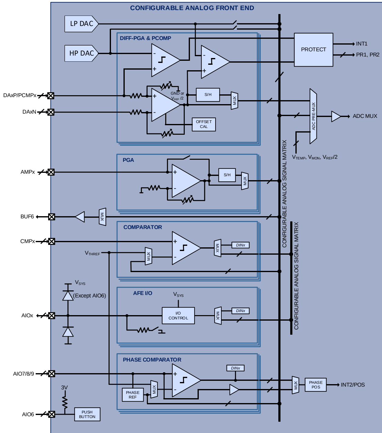
Figure 11-1 PAC52723 Configurable Analog Front End
