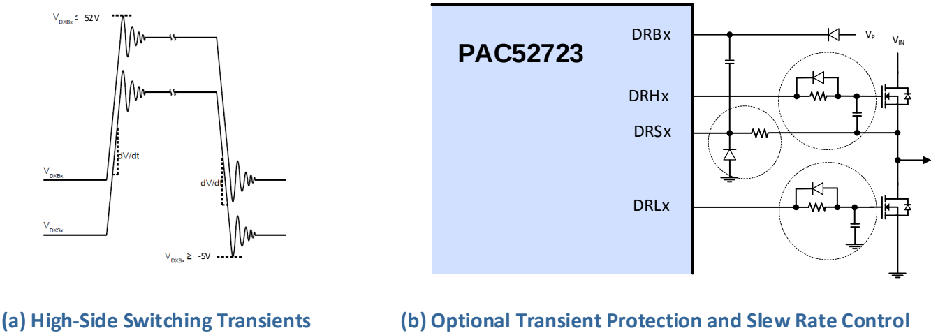
Figure 12-3 High-Side Switching Transients and Optional Circuitry
