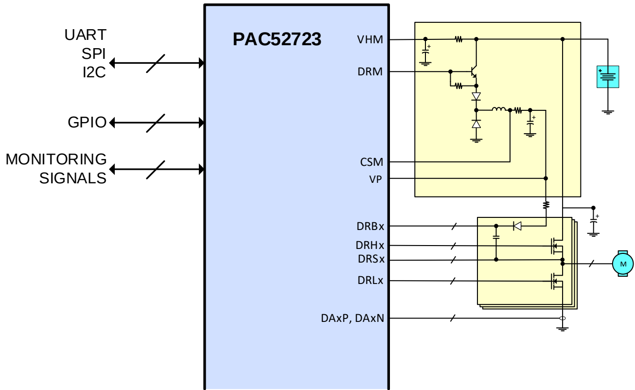
Figure 21-1 3-Phase Motor Drive Using PAC52723 (Simplified Diagram)
