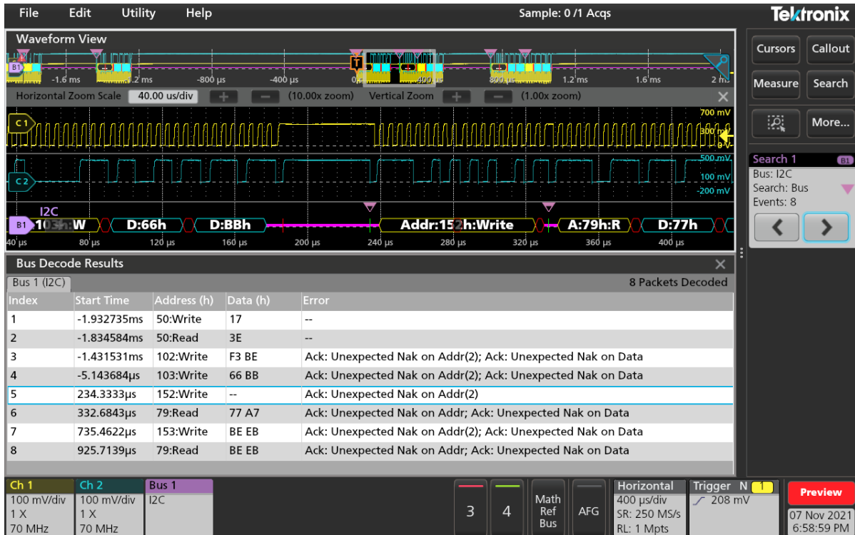
A bus waveform provides time-correlated decoded packets while the bus decode table presents all the packets from the entire acquisition, search can be used to navigate
