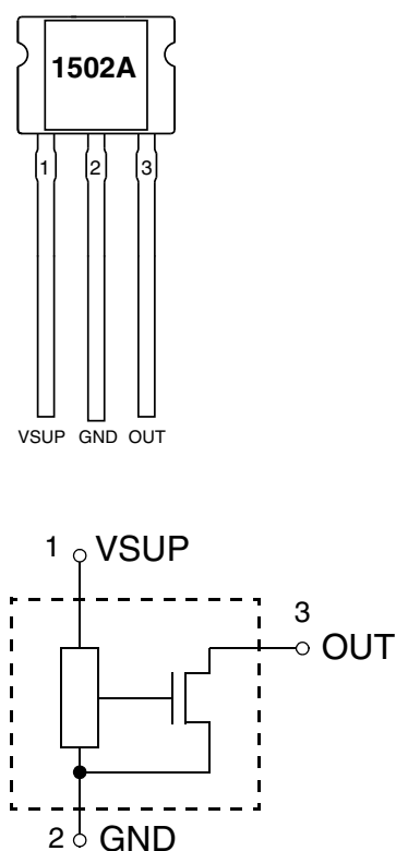
Fig. 4–5: Pin configuration
