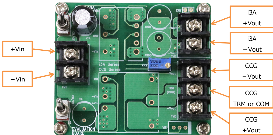
Fig.2-1 Outline
