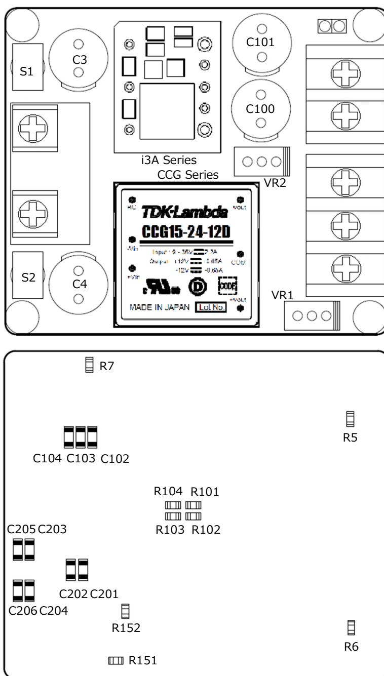
Fig.4-1 Component layout
