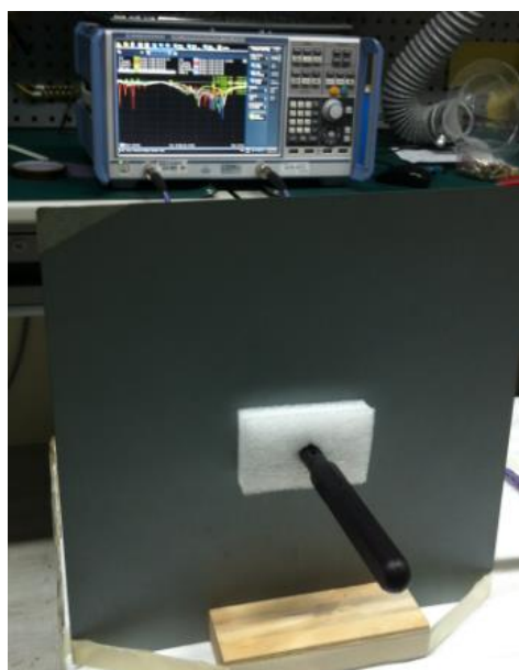
Antenna straight
