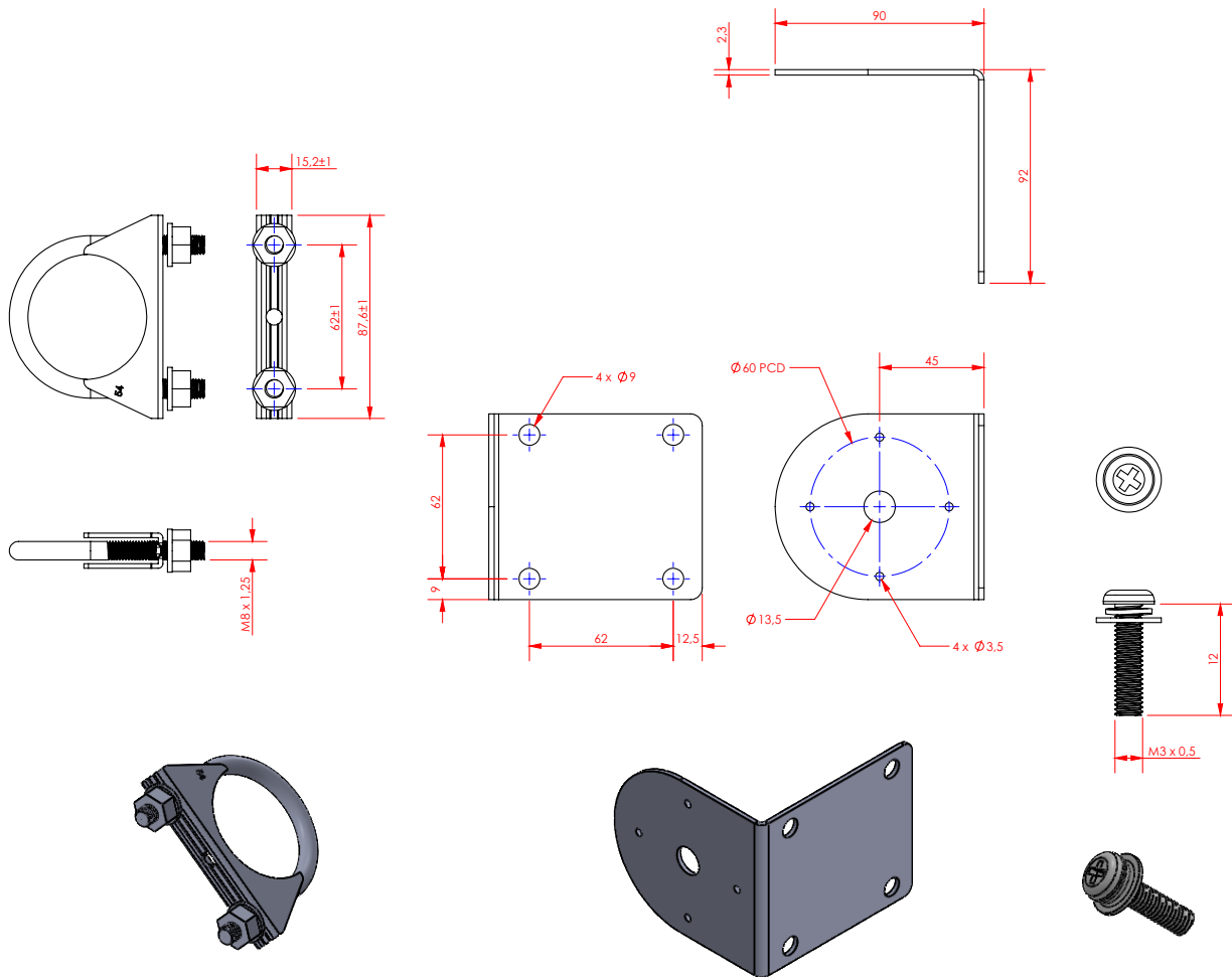
U-BOLT MAST CLAMP
