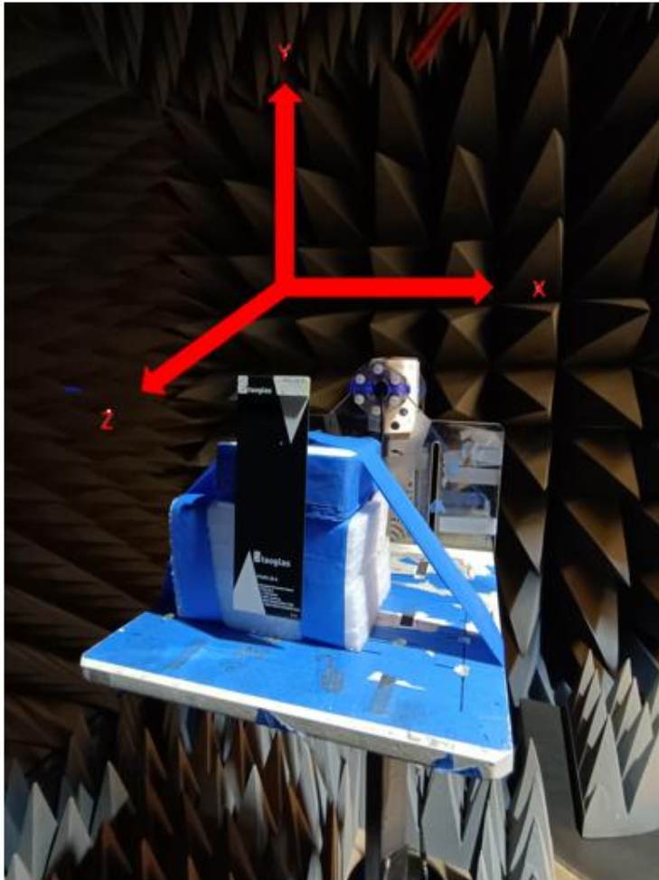
Chamber Setup
