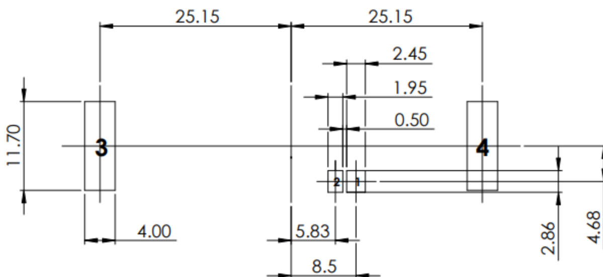
PCB FOOTPRINT
