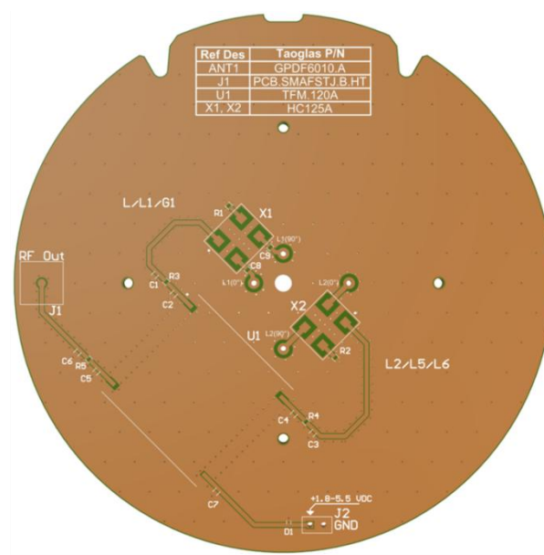
Bottom side ( TFM.120A placement including HC125A's )
