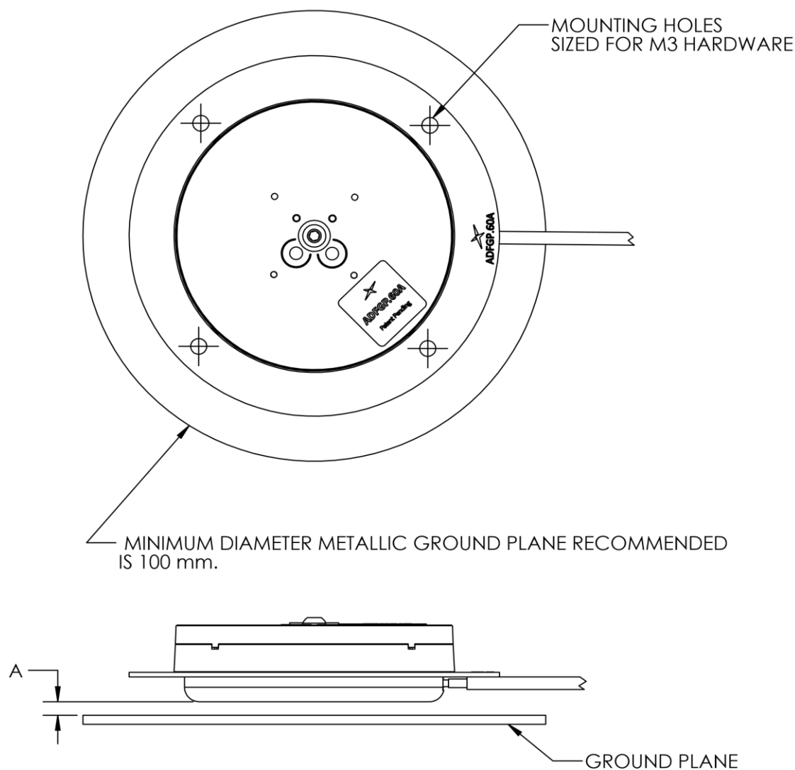
ANTENNA MOUNTING RECOMMENDATIONS
