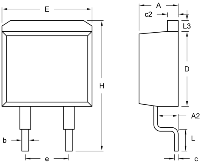
D 2 PAK-D
