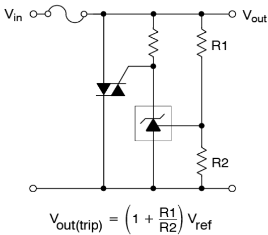
Figure 10: TRIAC Crowbar
