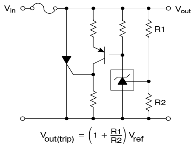
Figure 11: SCR Crowbar
