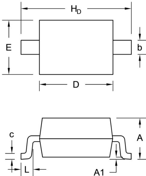
SOD-323
