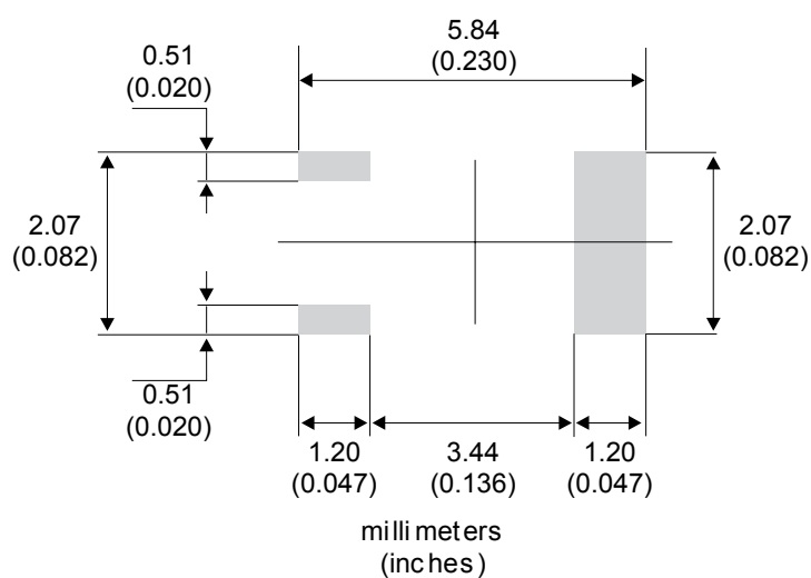
Figure 15. Footprint recommendations, dimensions in mm (inches)
