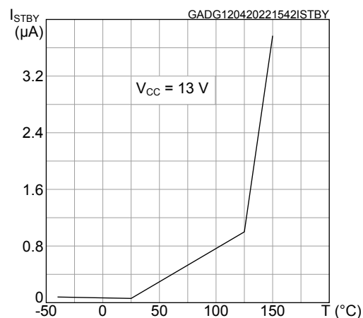
Figure 13. Standby current
