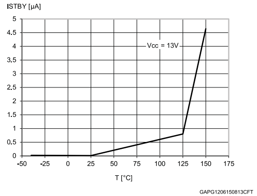
Figure 7: Standby current
