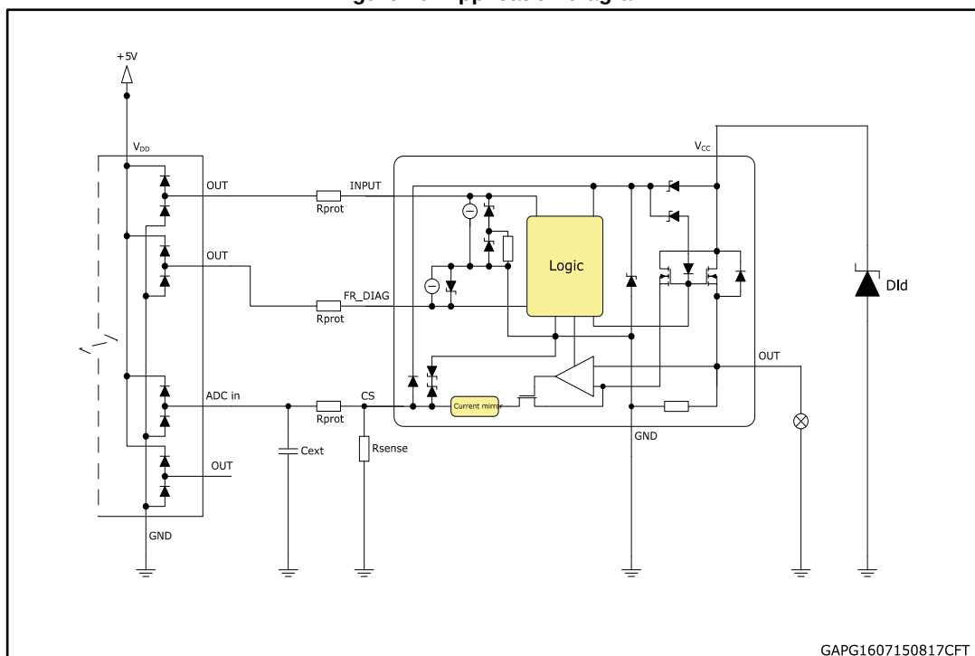
Figure 26: Application diagram
