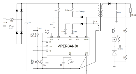
Figure 1. TYPICAL APPLICATION
