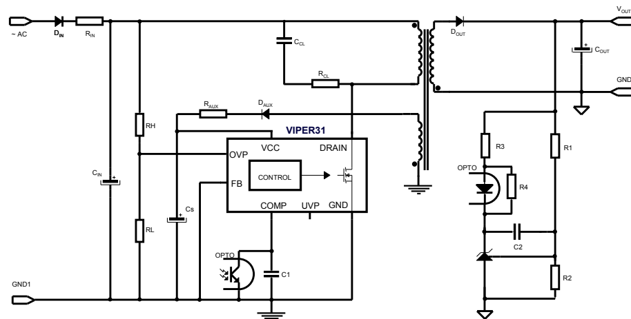
Figure 43. Flyback converter (isolated), with line OVP
