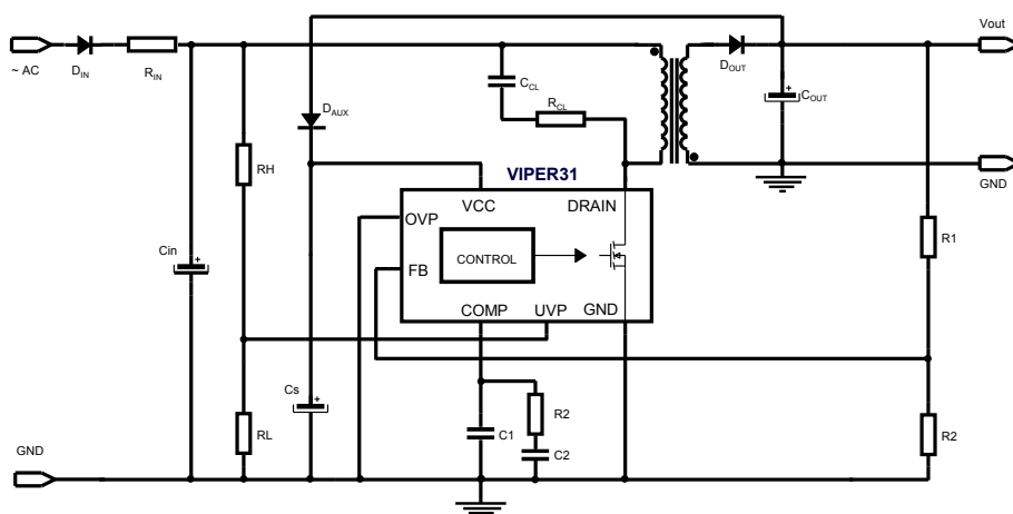
Figure 38. Flyback converter (non-isolated), with line UVP
