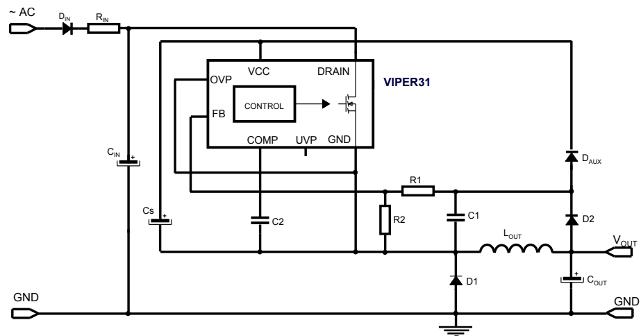
Figure 49. Buck converter
