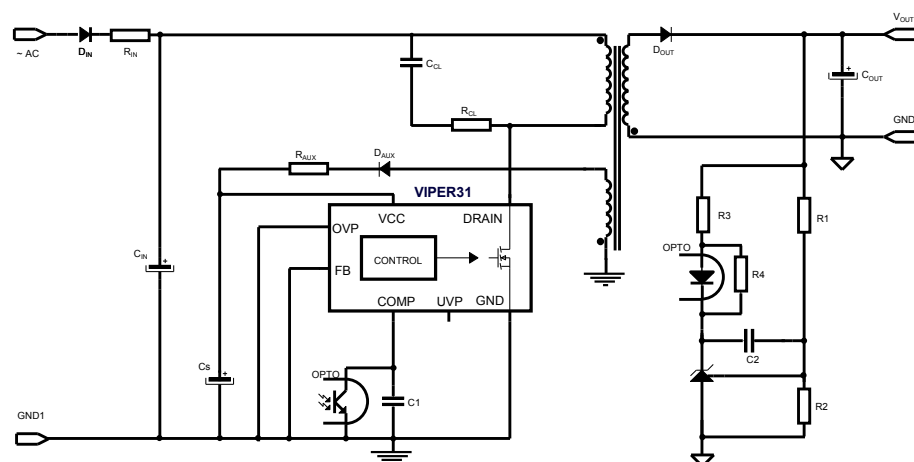
Figure 41. Flyback converter (isolated)
