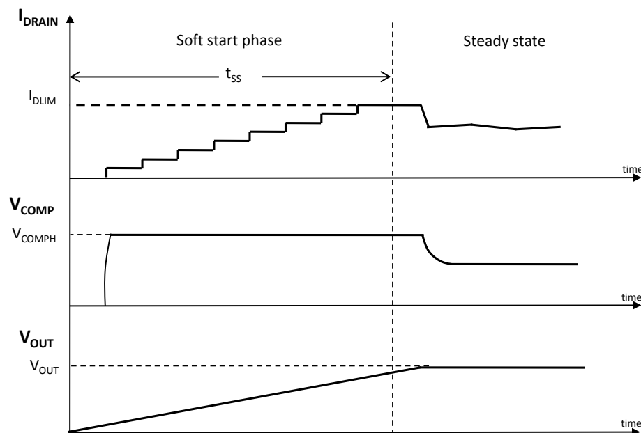
Figure 26. Soft startup
