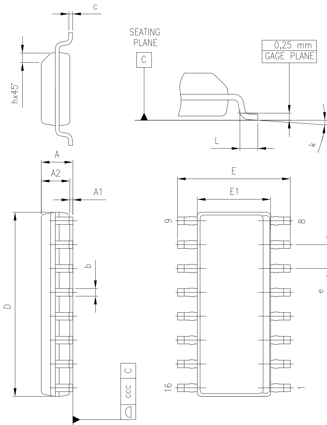
Figure 55. SO16N package outline
