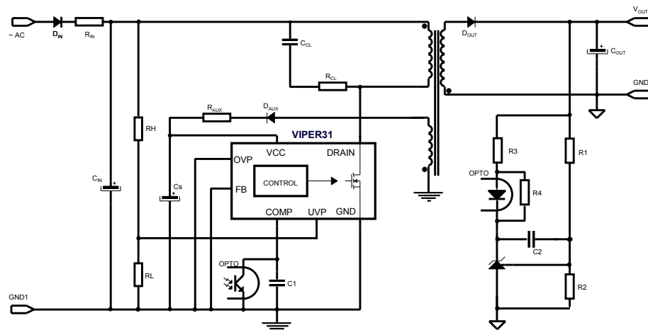
Figure 42. Flyback converter (isolated), with line UVP
