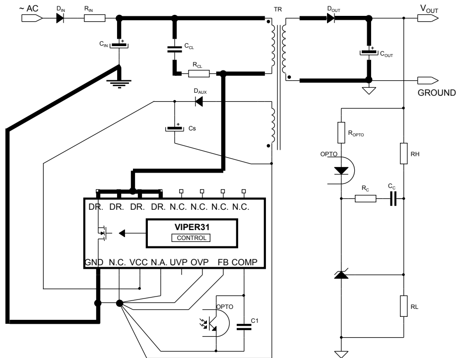
Figure 53. Recommended routing for flyback converter
