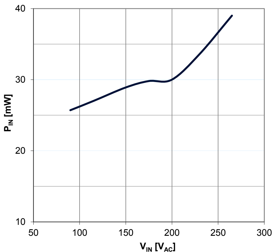
Figure 51. P_{IN} versus V_{IN} in no-load, V_{OUT} = 15\text{ V}
