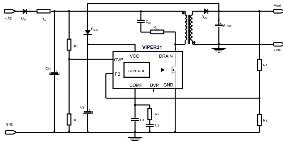
Figure 39. Flyback converter (non-isolated), with line OVP
