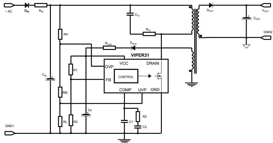
Figure 48. Flyback converter (primary regulation) with line UVP/OVP
