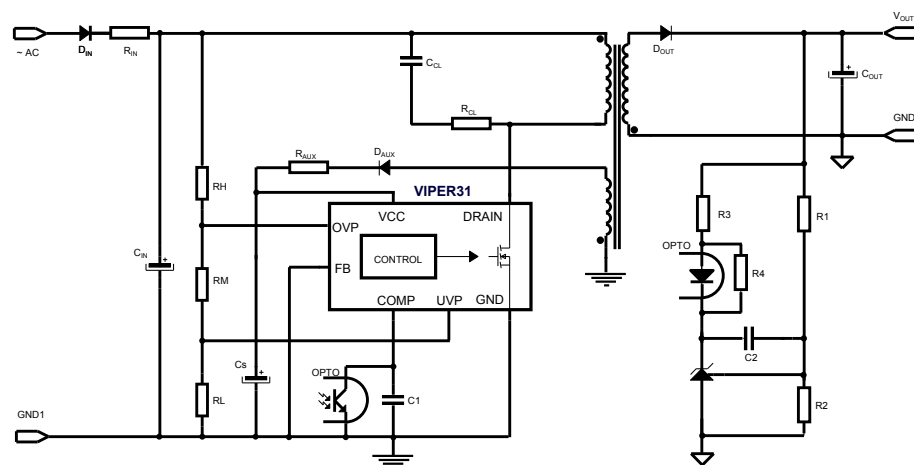
Figure 44. Flyback converter (isolated), with line OVP/UVP
