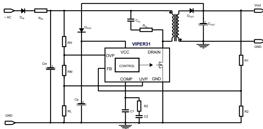
Figure 40. Flyback converter (non-isolated), with line UVP/OVP
