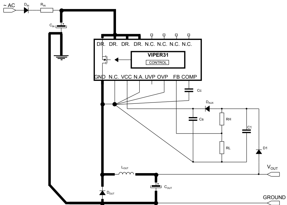
Figure 54. Recommended routing for buck converter
