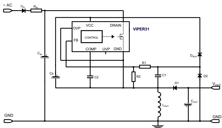
Figure 50. Buck-boost converter
