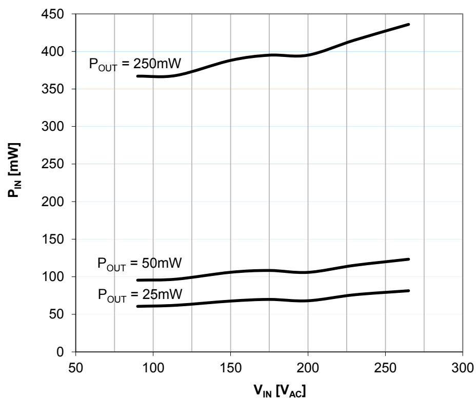
Figure 52. P_{IN} versus V_{IN} in light-load, V_{OUT} = 15V
