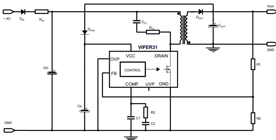
Figure 37. Flyback converter (non-isolated)
