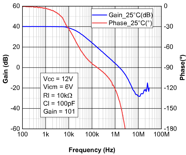
Figure 14. Bode diagram at V_{CC} = 12\text{ V}
