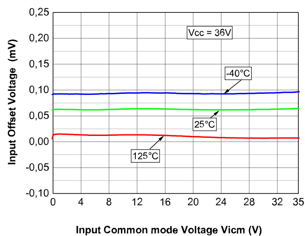
Figure 9. Input offset voltage vs. common-mode voltage at V_{CC} = 36\text{ V}
