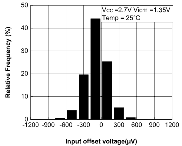
Figure 3. Input offset voltage distribution at V_{CC} = 2.7\text{ V}
