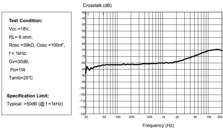
Figure 39. Crosstalk vs. frequency
