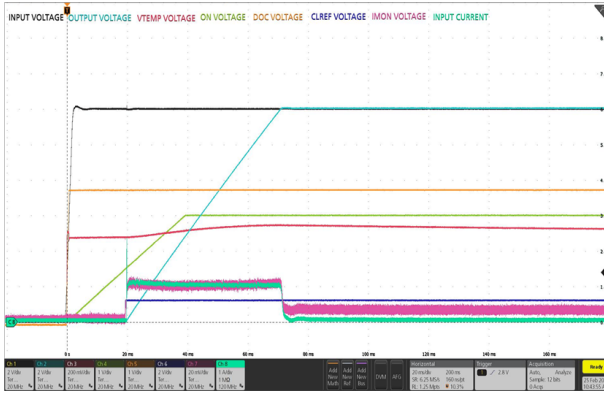
Figure 26. Startup by V_{IN} ( C_{OUT} = 6200\text{ }\mu\text{F} , no load)
