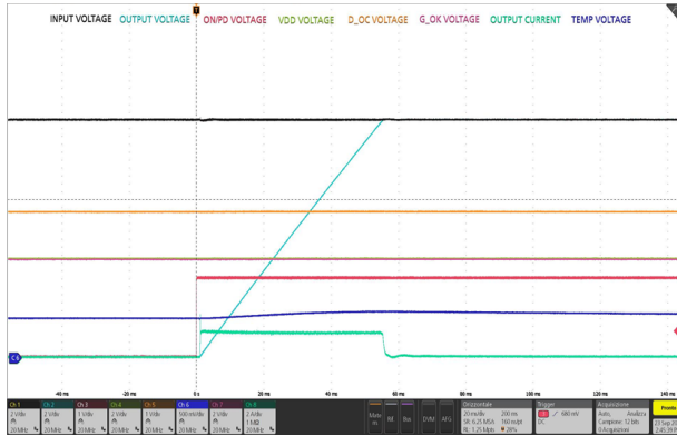
Figure 30. Startup by ON/PD ( I_{OUT} = 15\text{ A} , C_{OUT} = 6800\text{ }\mu\text{F} )
