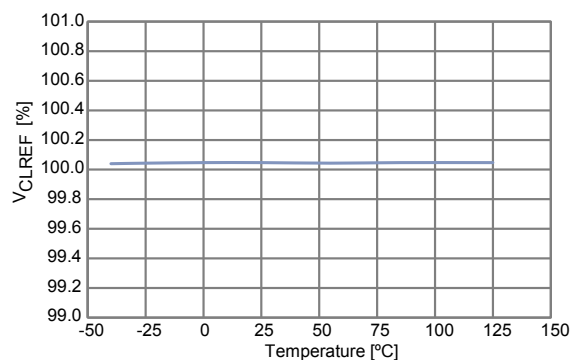
Figure 13. V_{CLREF} threshold vs. temperature
