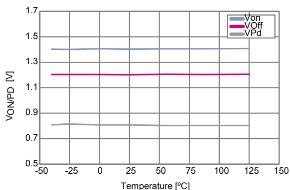
Figure 18. ON/PD thresholds vs. temperature
