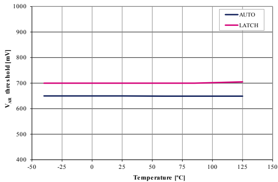
Figure 17. Auto pin thresholds vs. temperature
