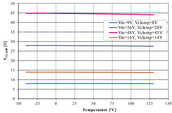
Figure 15. Clamping voltage vs. temperature
