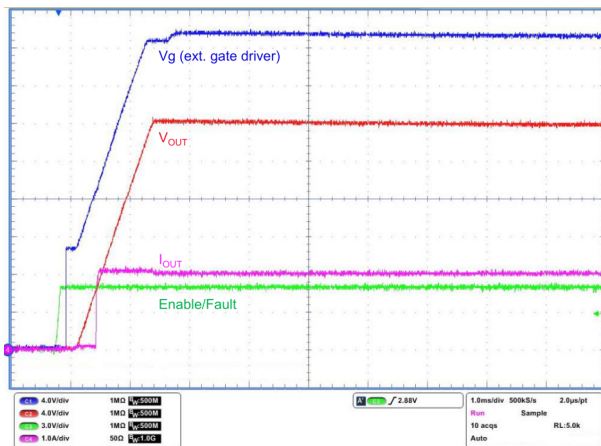
Figure 35. Enable turn-on with external FET
