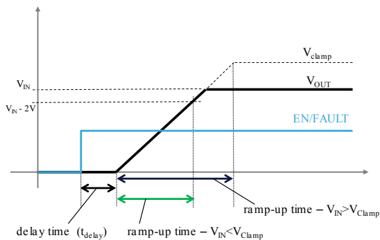
Figure 11. Startup time
