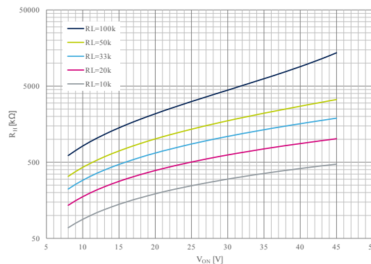
Figure 6. UVLO threshold ( V_{ON} ) vs R_H , R_L
