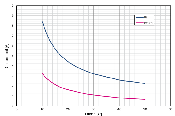
Figure 28. Current limit vs. R_limit (zoom)
