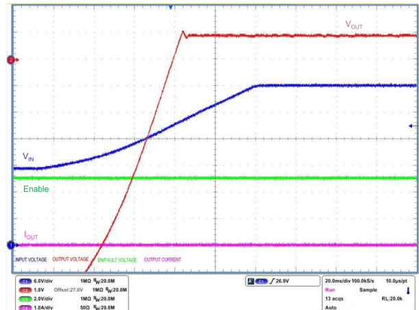
Figure 30. V_{OUT} clamping (28 V)
