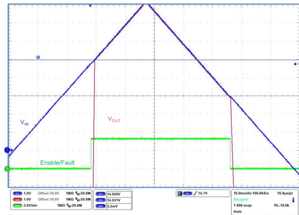
Figure 34. UVLO
