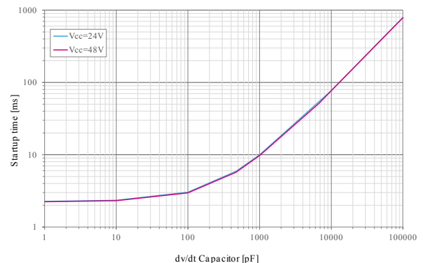
Figure 12. Startup time vs C_{dv/dt}
