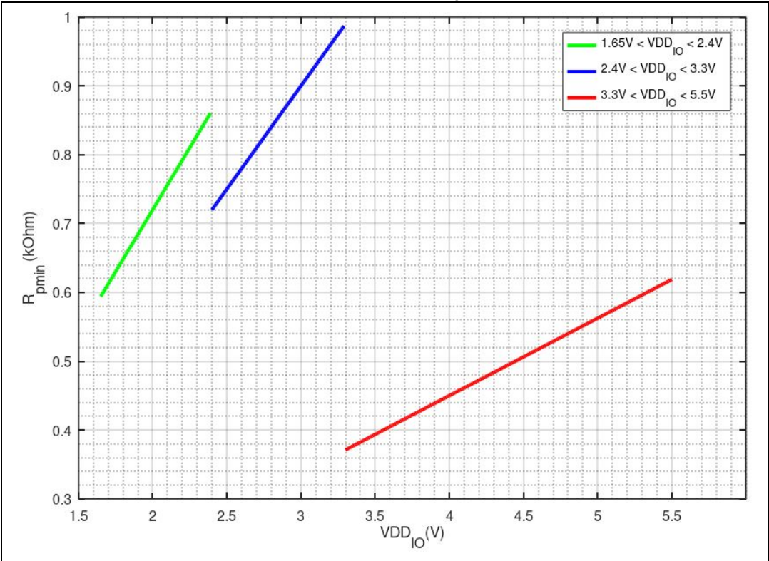
Figure 30. R_{Pmin} vs. V_{DD} , f_c = 3.4 MHz
