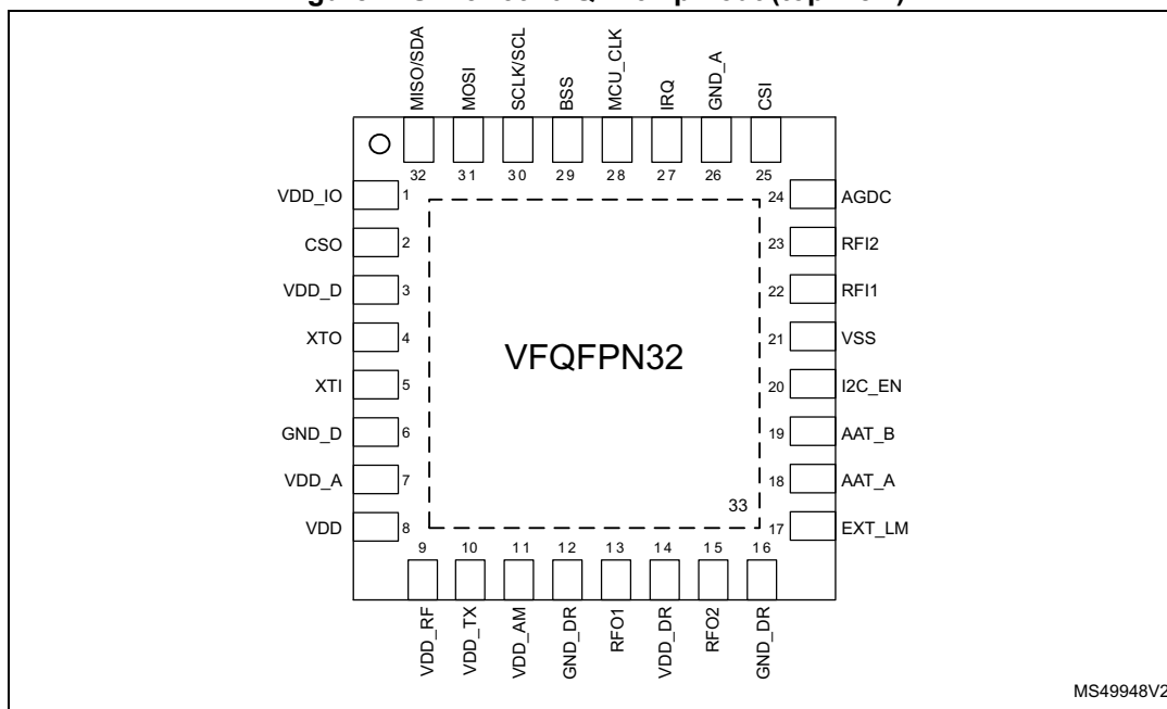
Figure 4. ST25R3920 QFN32 pinout (top view)
