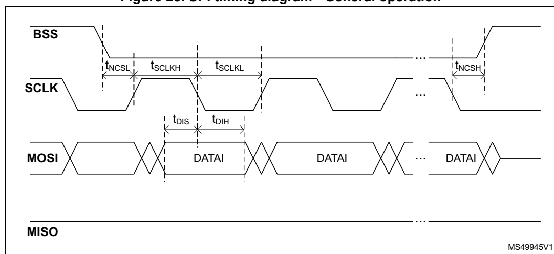
Figure 28. SPI timing diagram - General operation
