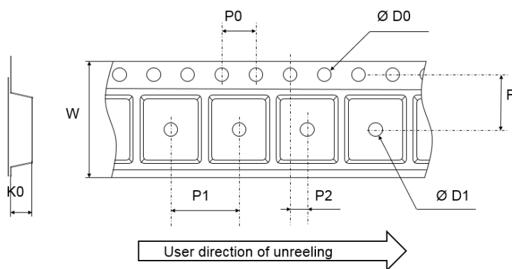
Figure 23. Tape outline
