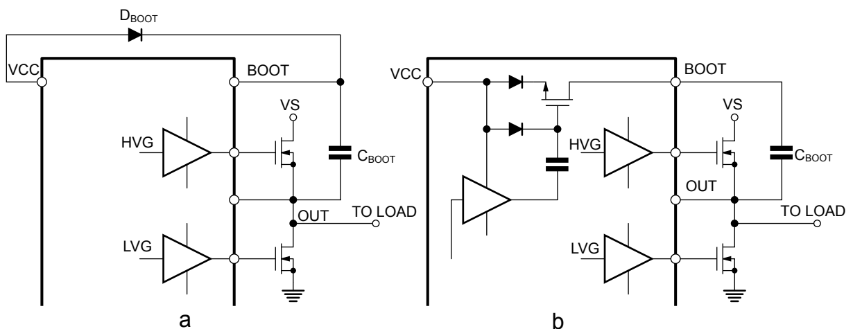
Figure 16. Bootstrap structure
