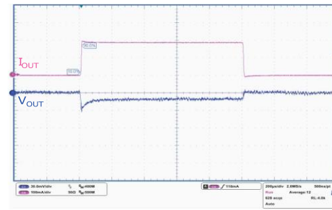
Figure 27: Load transient ( V_{OUT} = 5\text{ V} )
