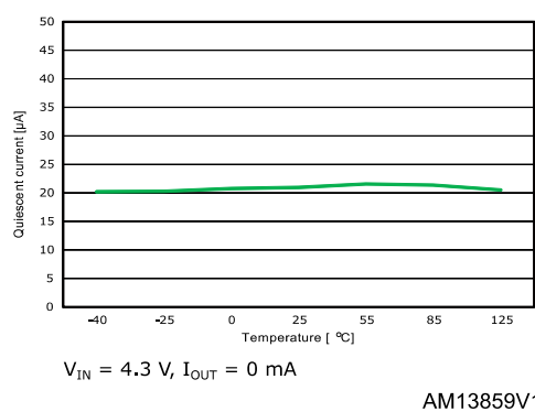
Figure 8: Quiescent current vs temperature ( I_{OUT} = 0 \text{ mA} )
