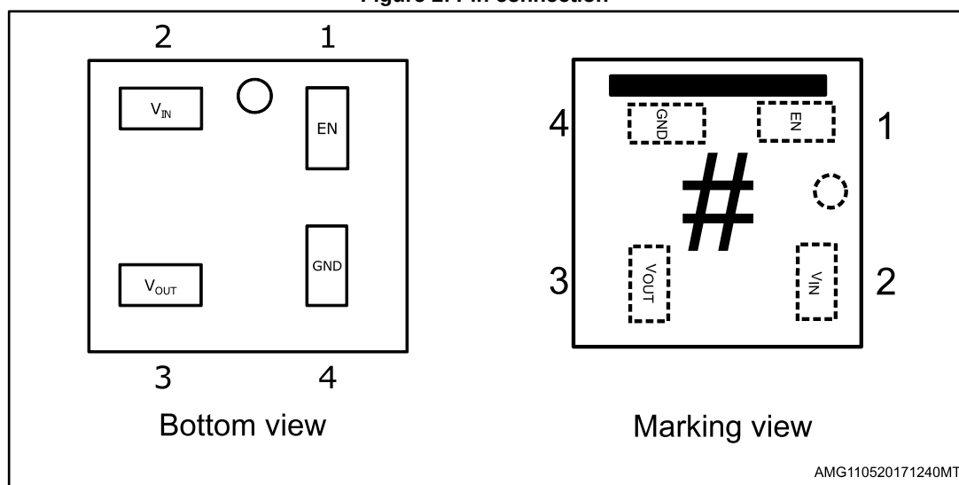
Figure 2: Pin connection
