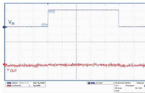
Figure 25: Line transient ( V_{OUT} = 5\text{ V} )
