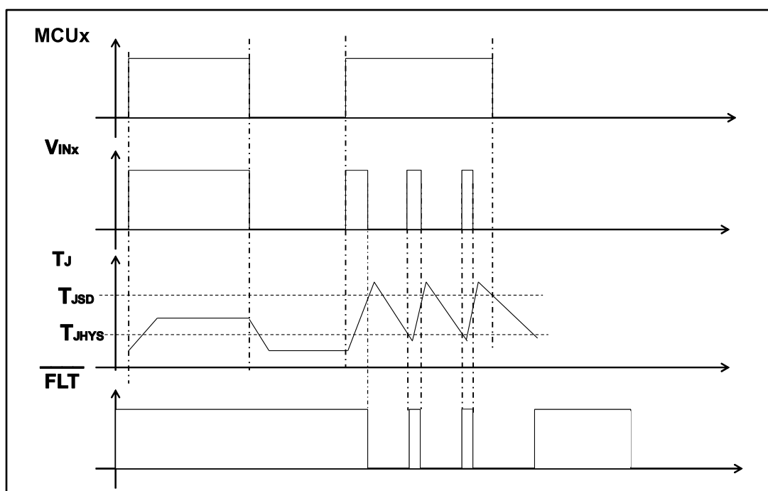
Figure 8: Thermal protection signalization behavior on FLT
