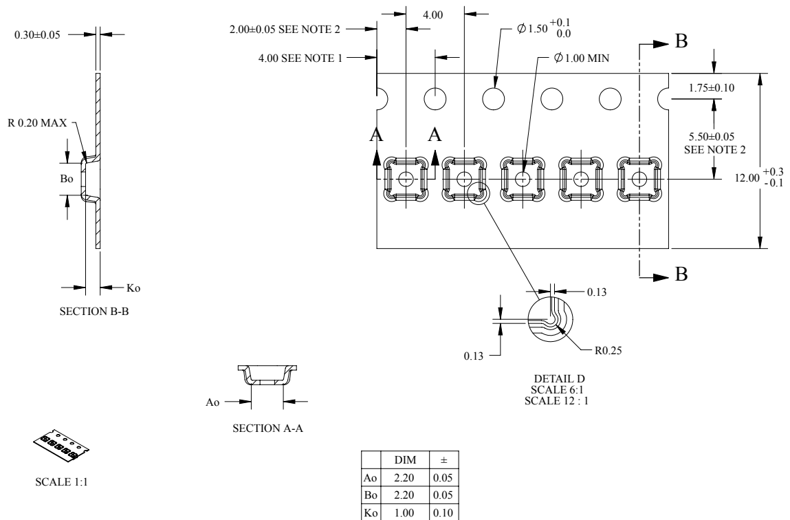
Figure 25. Carrier tape information for HLGA-10L package
