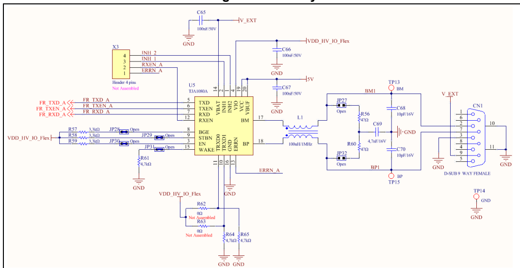
Figure 8. FlexRay
