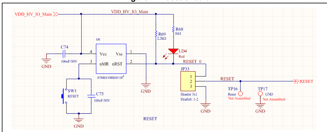
Figure 7. Reset circuit
