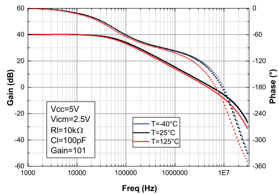
Figure 22. Bode diagram at V_{CC} = 5\text{ V}
